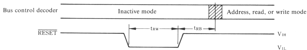
Fig. 6 Reset timing
