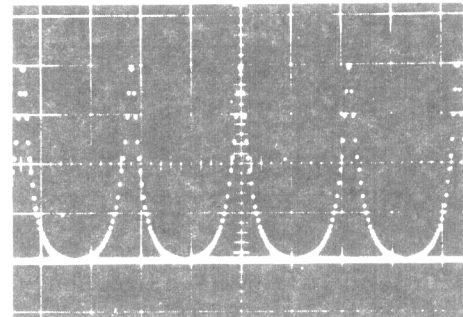
Fig. 2 Output waveform of single tone with envelope (RE = XXXX110)
