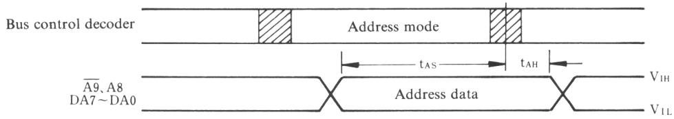
Fig. 7 Address timing
