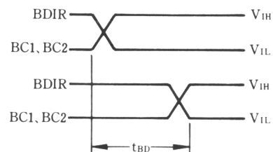
Fig. 5 Bus control timing
