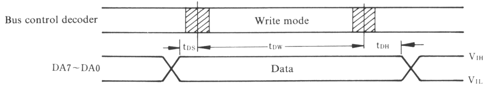
Fig. 8 Write mode
