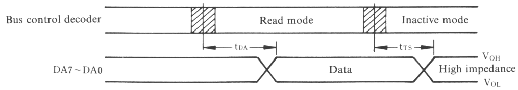
Fig. 9 Read mode
