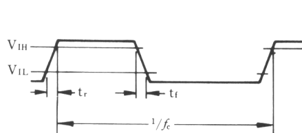
Fig. 4 Clock timing
