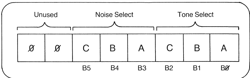
Figure 7.3 Register 7 – mixer/channel select register
