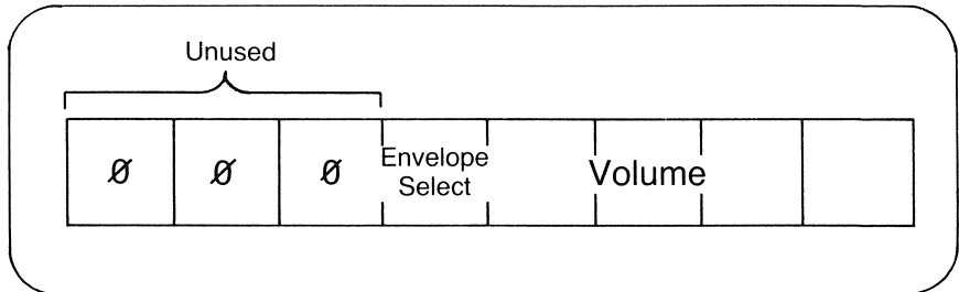
Figure 7.4 The volume control registers
