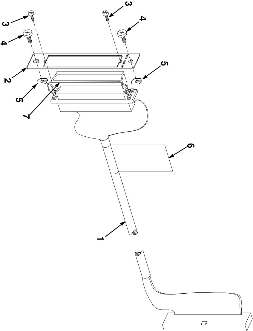
Figure 8. Cable Assembly, Internal SCSI
